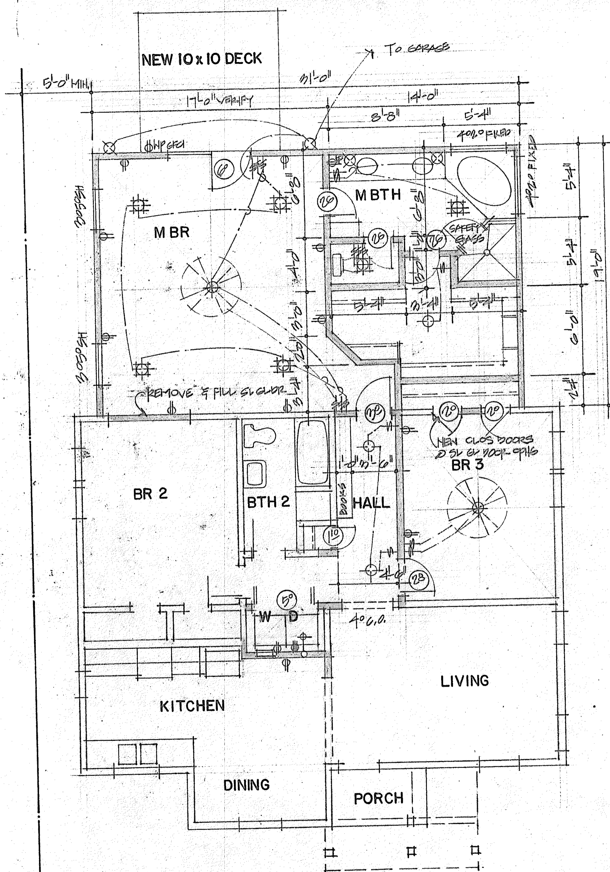
1/4" REMODEL/ADDITION FLOOR PLAN VERIFY ALL DIMENSIONS & CONDITIONS @ SITE ADDITION CUB & FLOOR HEIGHTS TO MATCH EXISTING. VERIFY LOCATIONS OF ALL ELECTRICAL SWITCHES, LIGHTS, FIXTURES @ SITE W/ OWNER. PROVIDE SERVICE FOR HVAC & WH IN ATTIC
